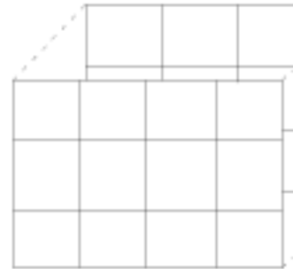
Result: 3-by-4-by-1
